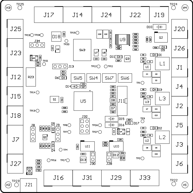
Top Assembly (Scale 1:1)
