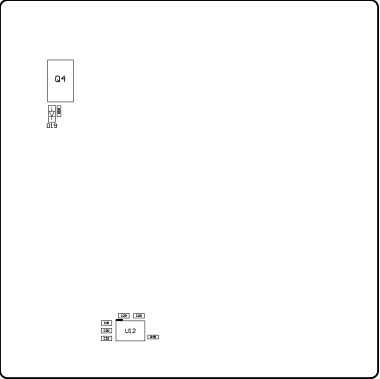
Bottom Assembly (Scale 1:1)
