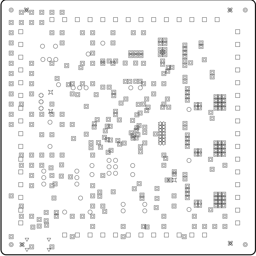
Drill Drawing View (Scale 1.28:1)
