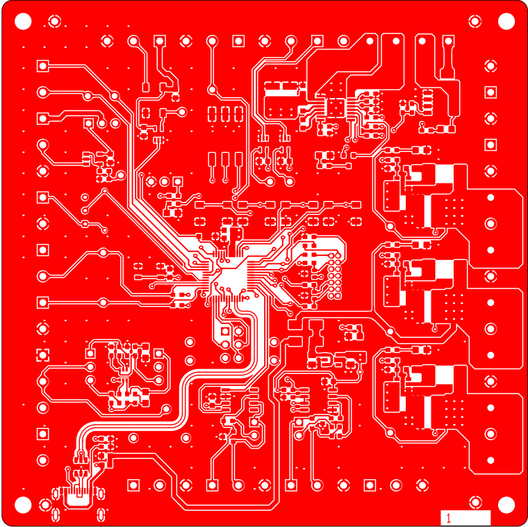
L1(Signal) (Scale 1:1)
