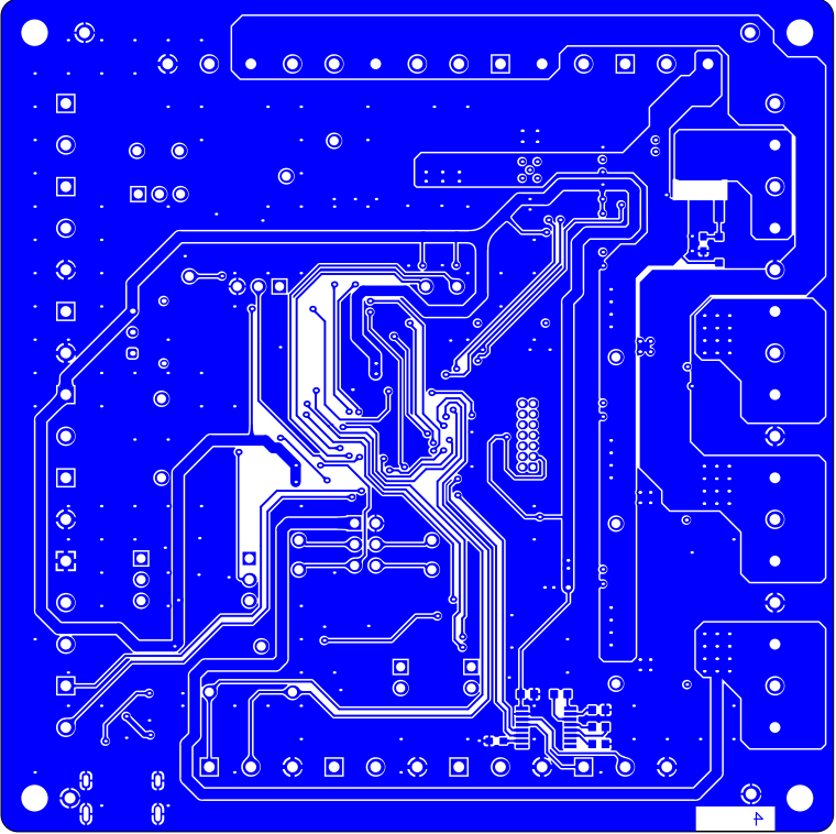
L4(Signal) (Scale 1:1)
