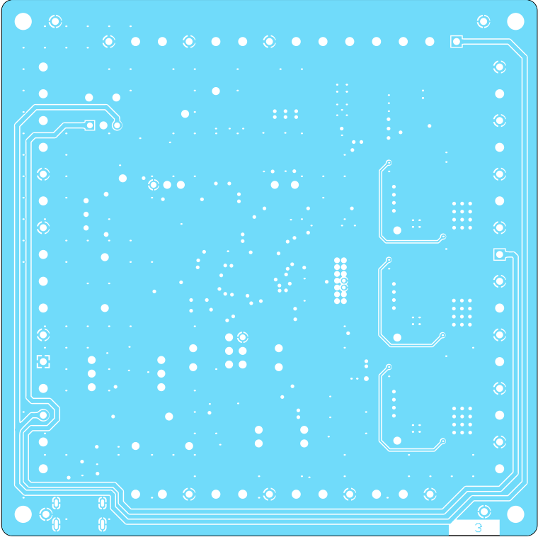
L3(GND) (Scale 1:1)
